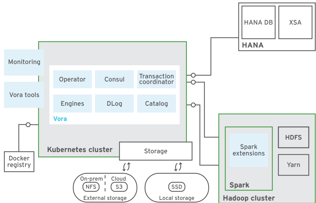
Figure 1. SAP Vora 2.0 Architecture
